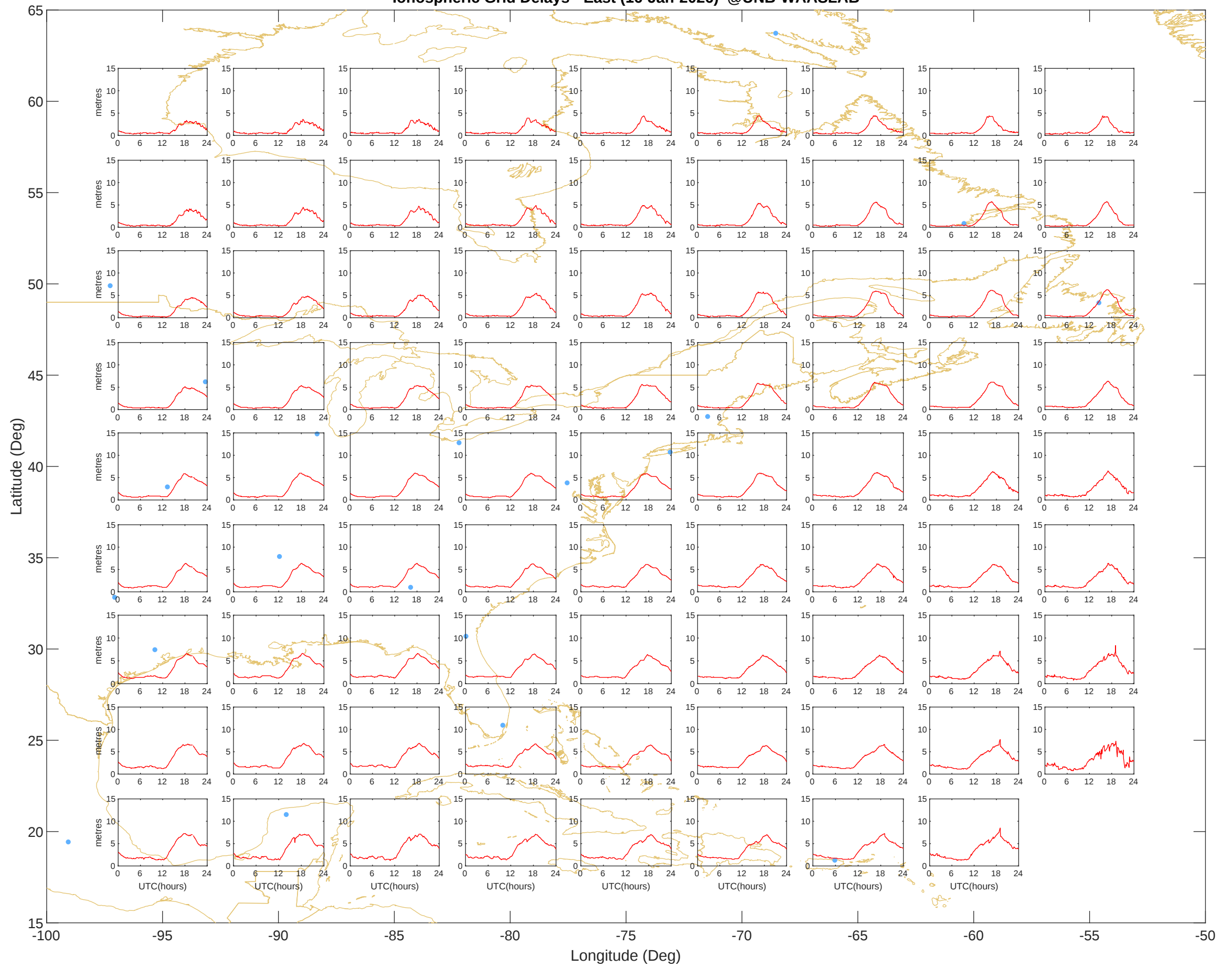
Ionospheric Grid Delays - East (16-Jan-2026) @UNB-WAASLAB
