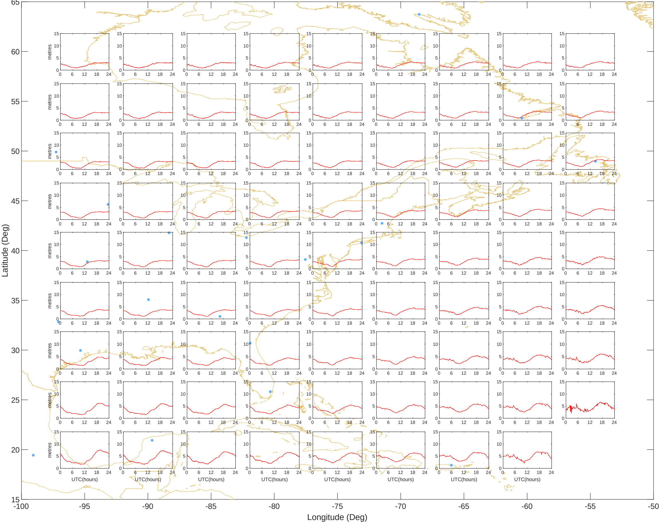
Ionospheric Grid Delays - East (31-Jul-2025) @UNB-WAASLAB
