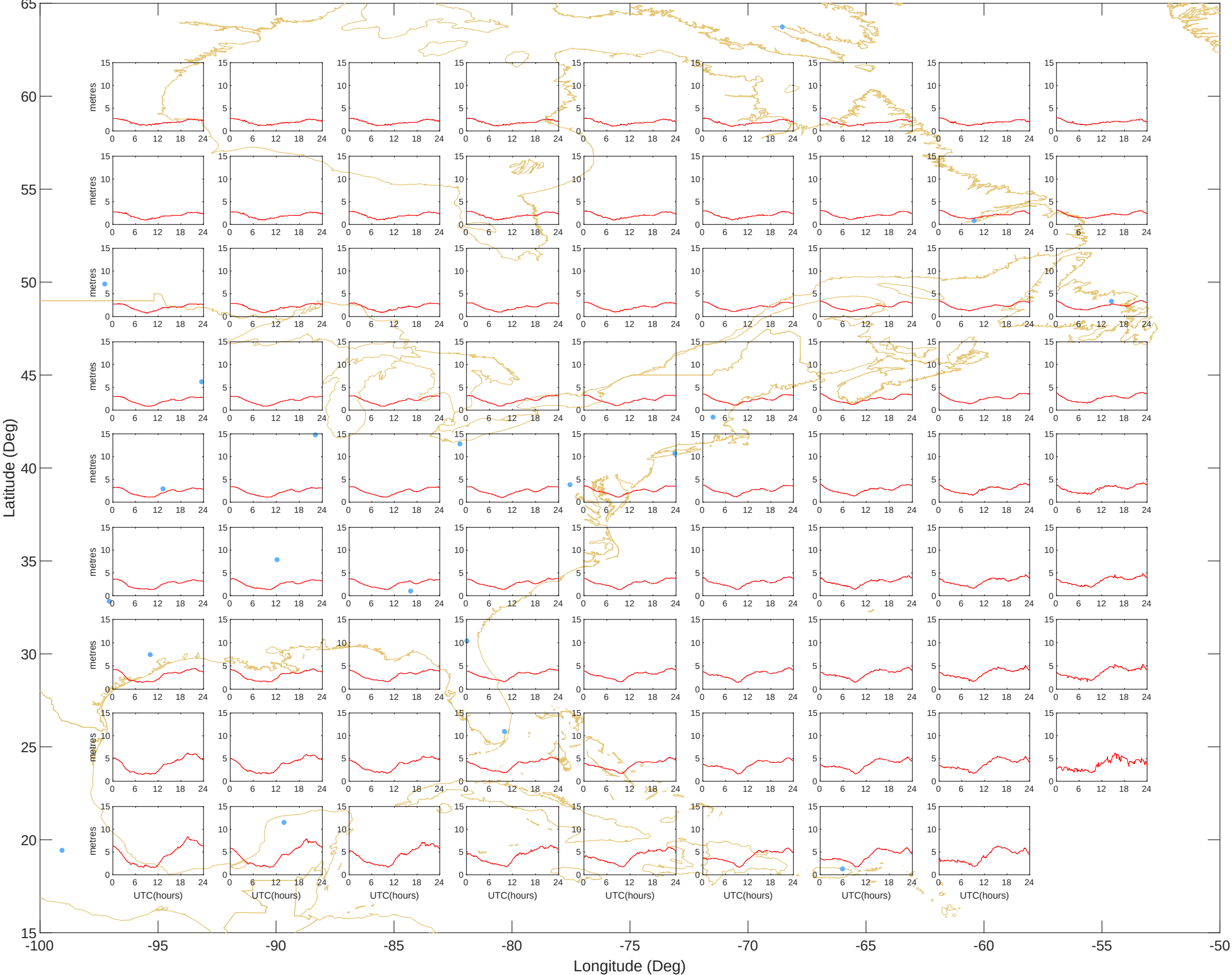
Ionospheric Grid Delays - East (11-Jul-2025) @UNB-WAASLAB
