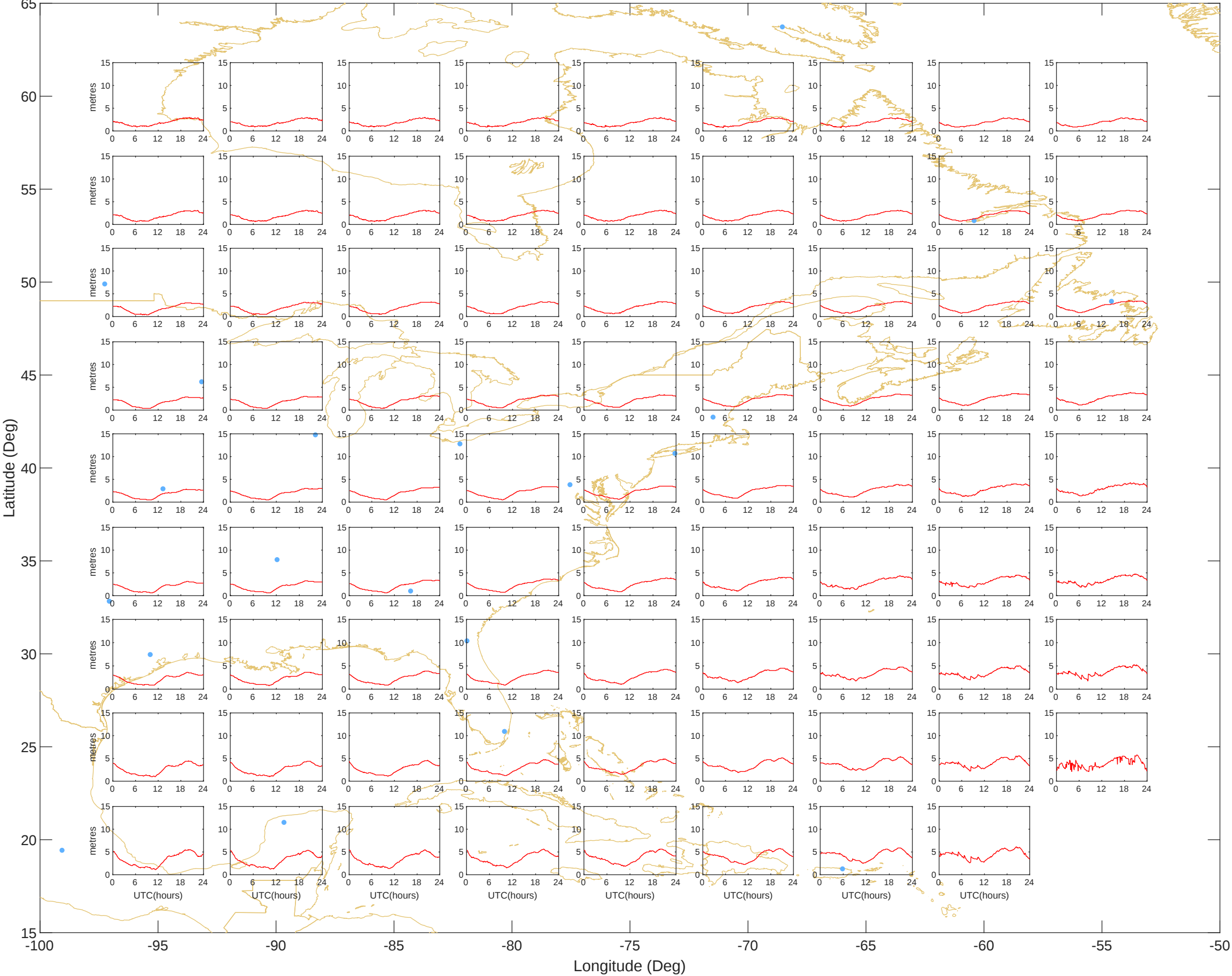
Ionospheric Grid Delays - East (08-Jul-2025) @UNB-WAASLAB
