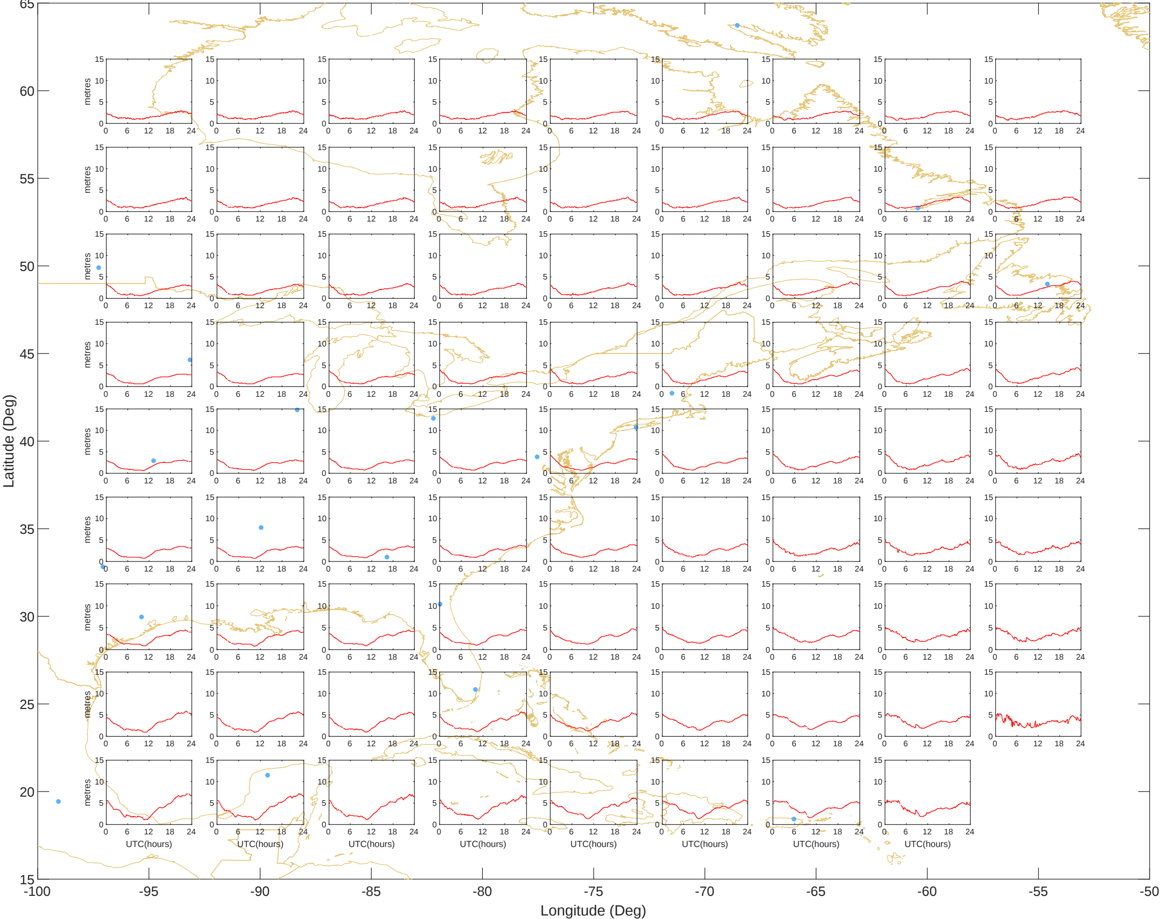
Ionospheric Grid Delays - East (05-Jul-2025) @UNB-WAASLAB
