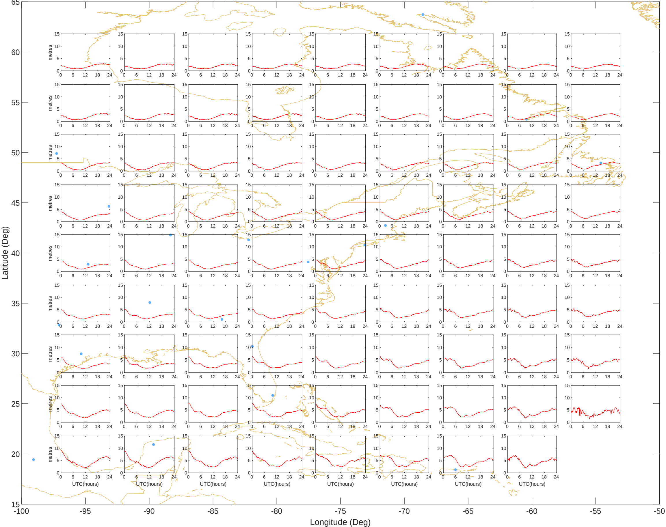
Ionospheric Grid Delays - East (04-Jul-2025) @UNB-WAASLAB
