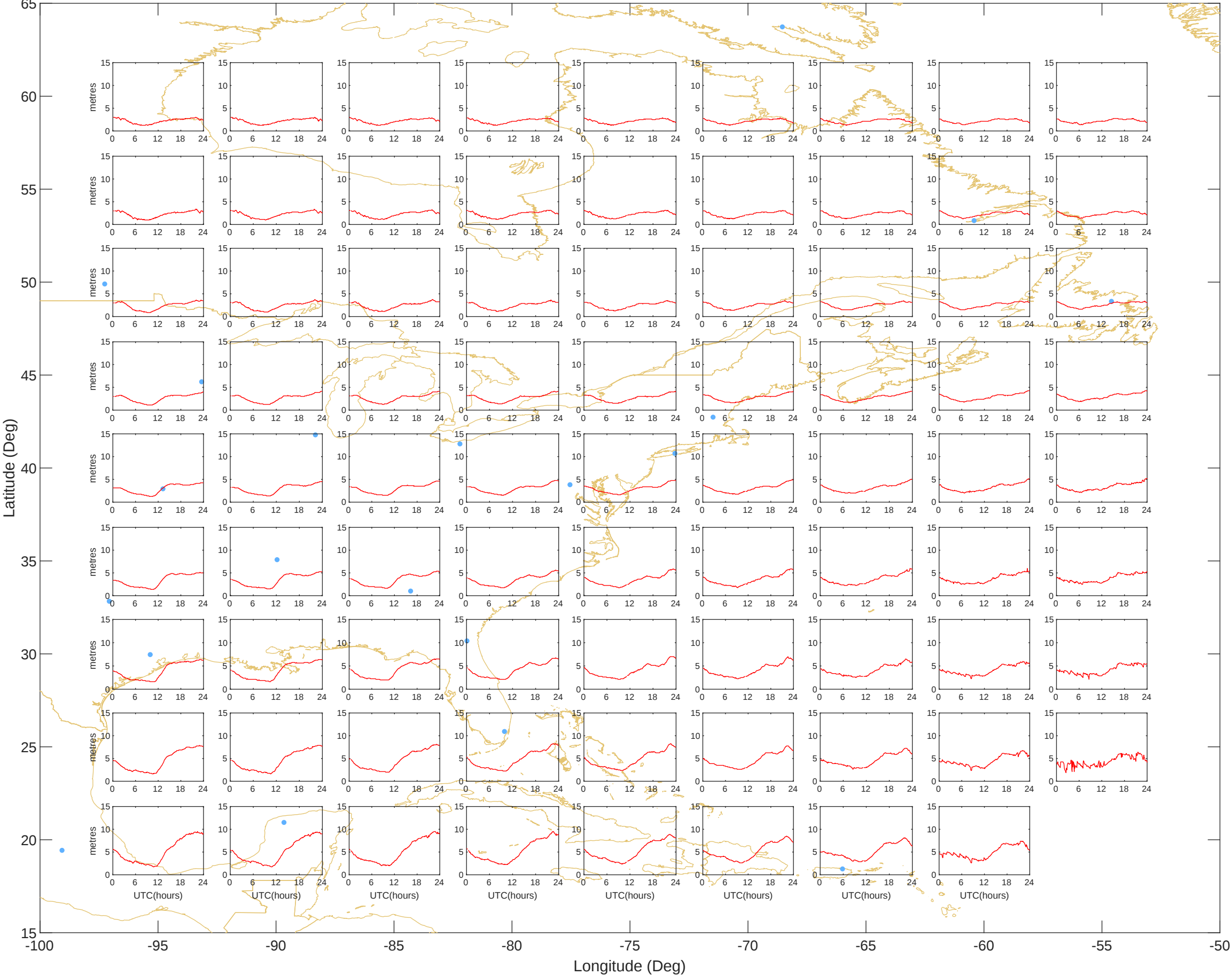
Ionospheric Grid Delays - East (03-Jul-2025) @UNB-WAASLAB
