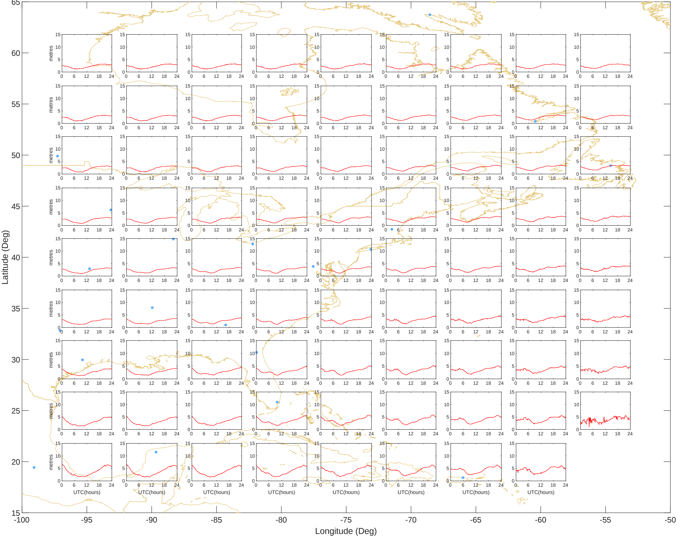
Ionospheric Grid Delays - East (02-Jul-2025) @UNB-WAASLAB
