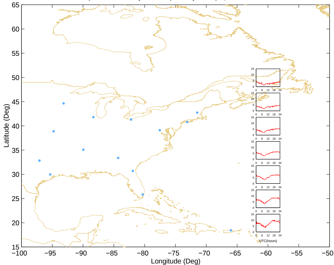
Ionospheric Grid Delays – East (29-May-2002) @UNB-WAASLAB
