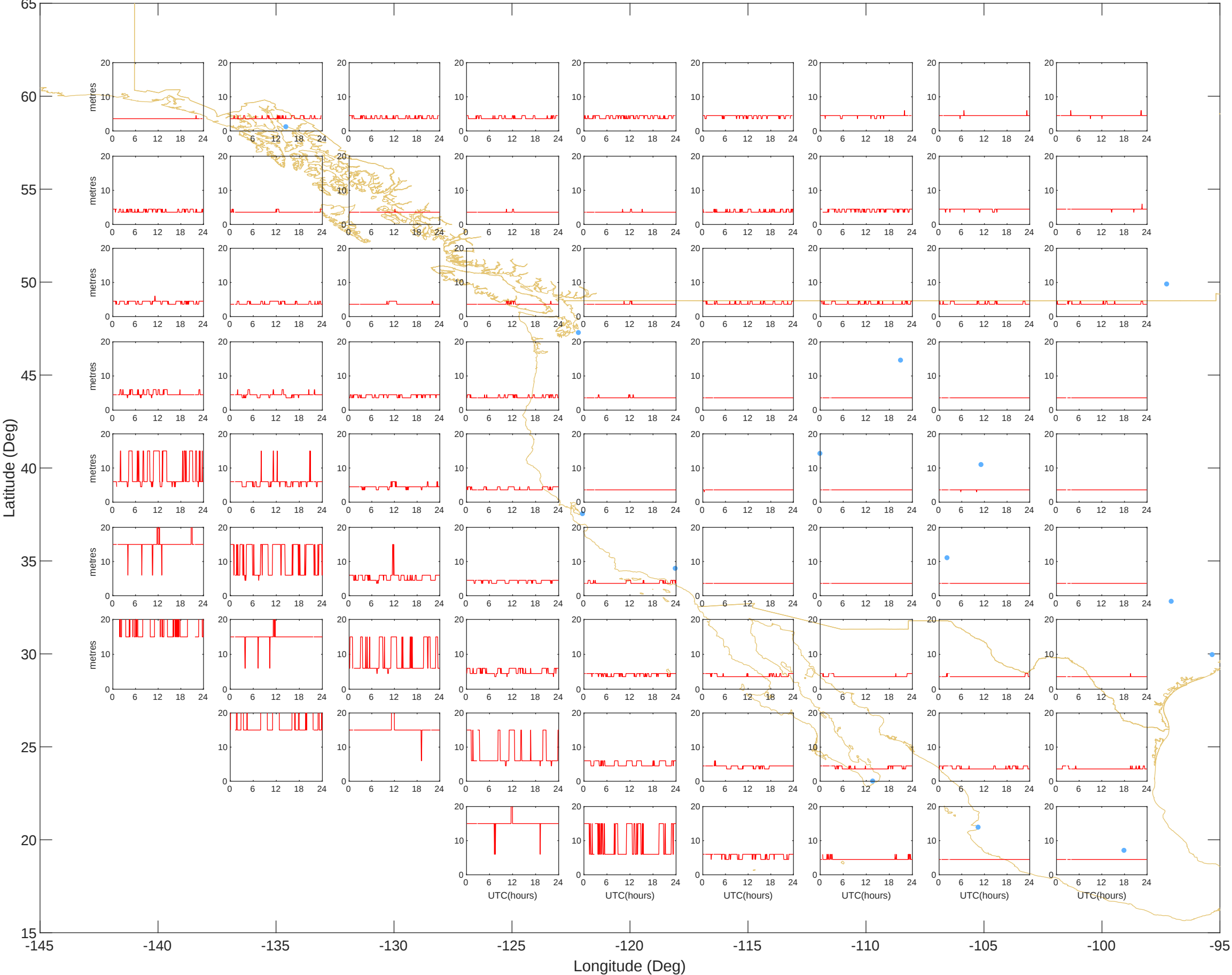
GIVEs - West (29-Jun-2026) @UNB-WAASLAB
