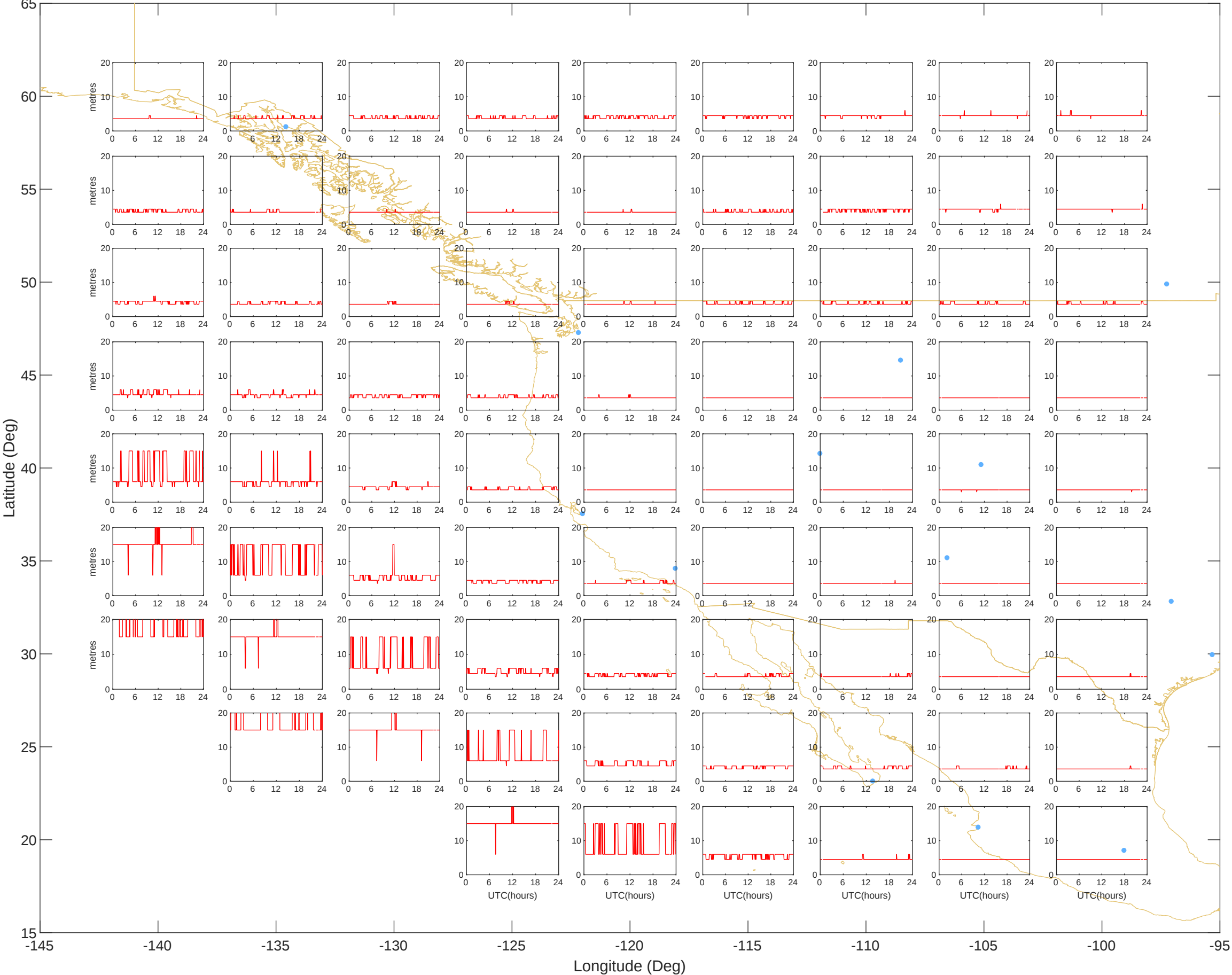
GIVEs - West (28-Jun-2026) @UNB-WAASLAB
