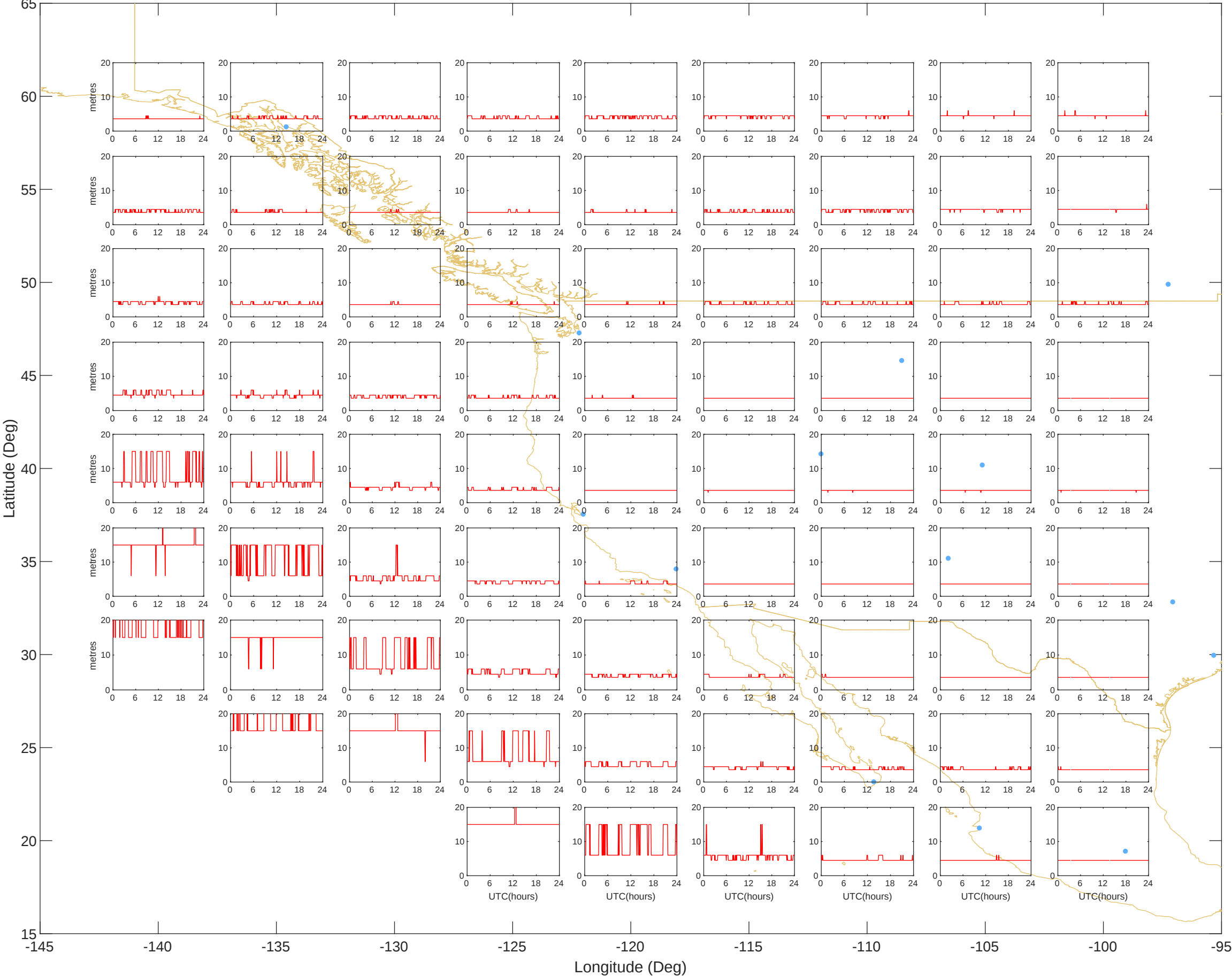
GIVEs - West (17-Jun-2026) @UNB-WAASLAB
