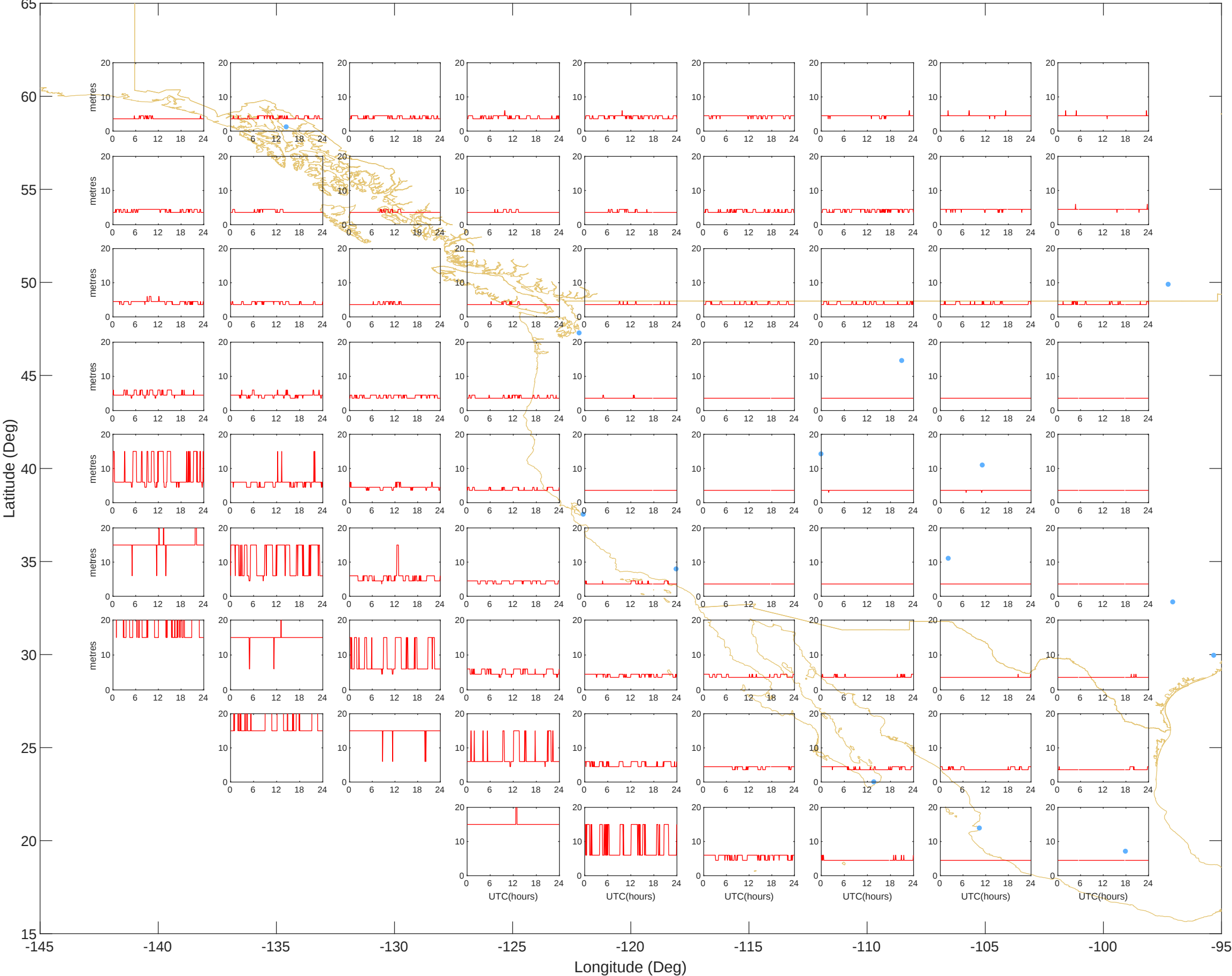
GIVEs - West (14-Jun-2026) @UNB-WAASLAB
