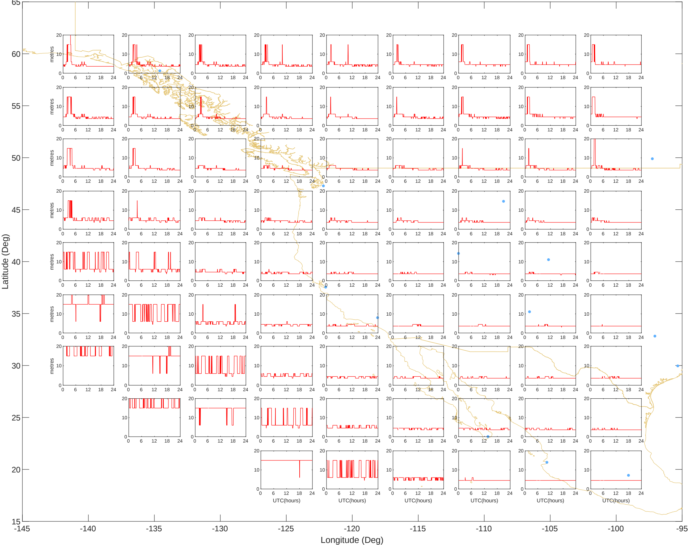
GIVEs - West (14-Mar-2026) @UNB-WAASLAB
