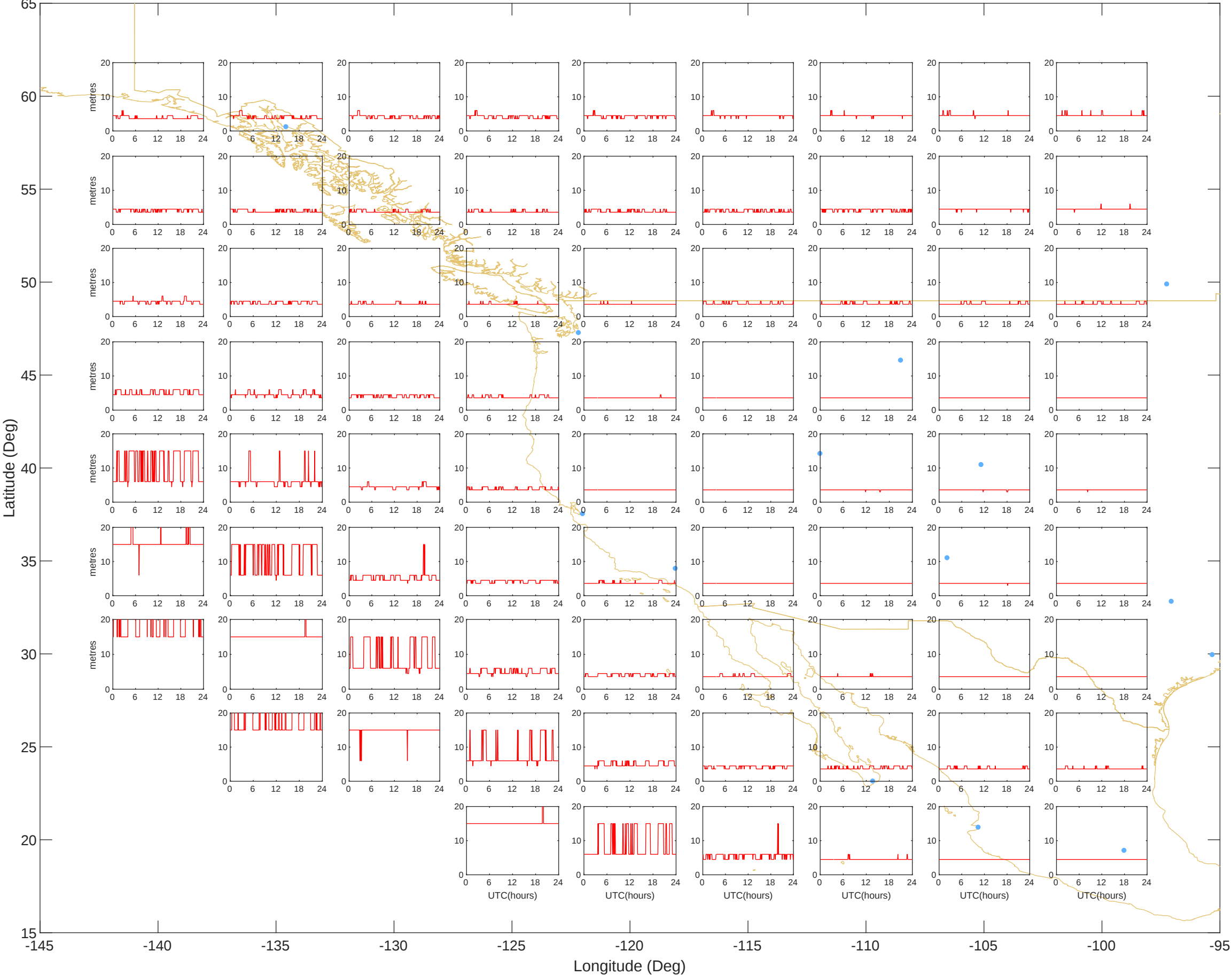
GIVEs - West (01-Mar-2026) @UNB-WAASLAB
