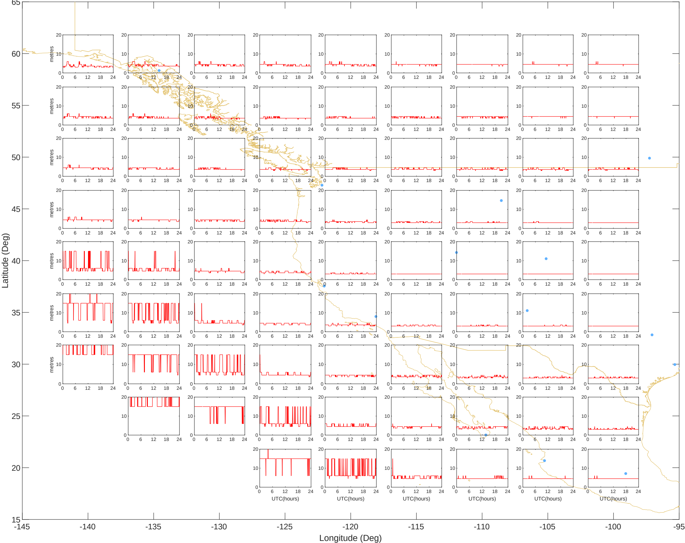
GIVEs - West (08-Nov-2025) @UNB-WAASLAB
