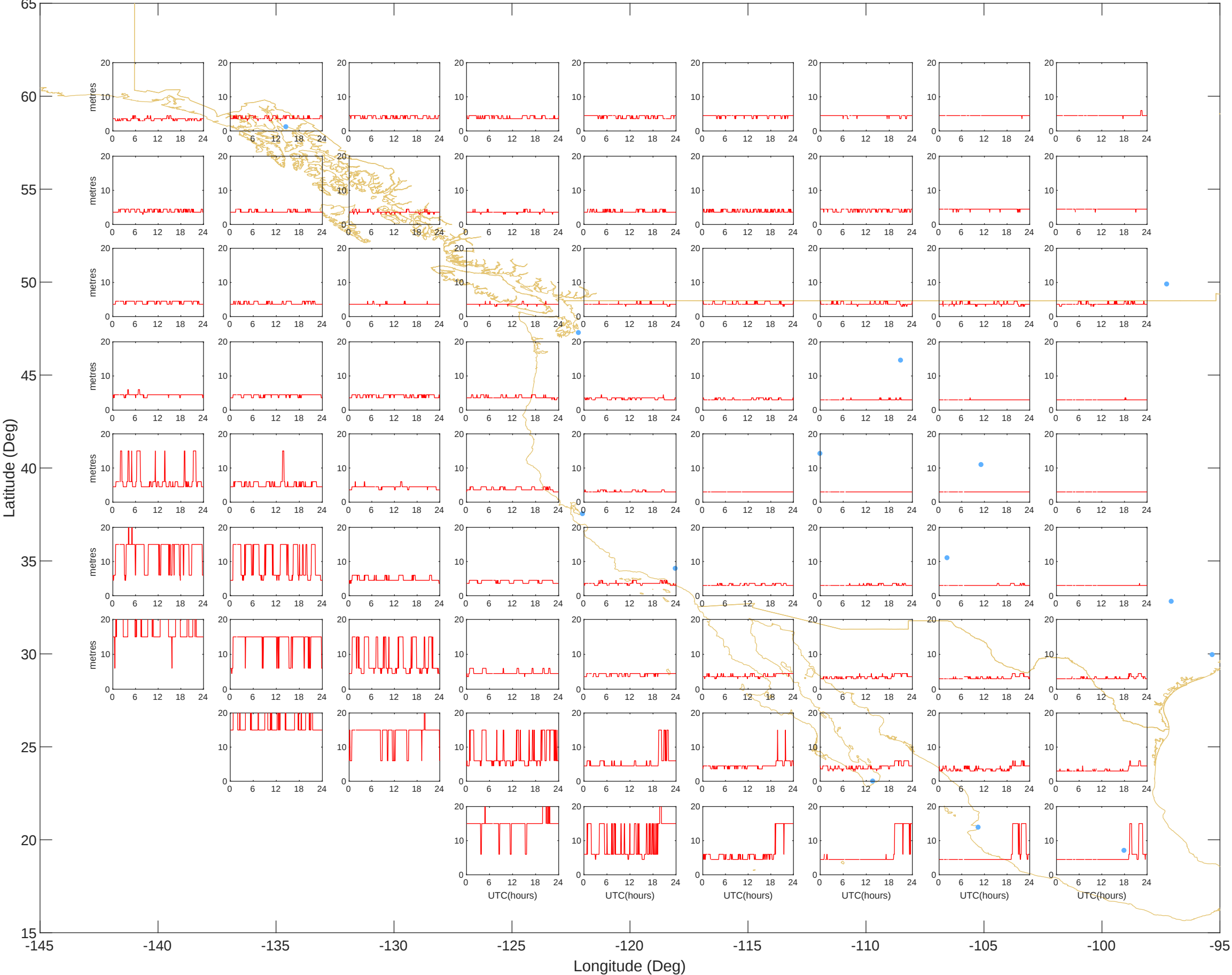
GIVEs - West (25-Oct-2025) @UNB-WAASLAB
