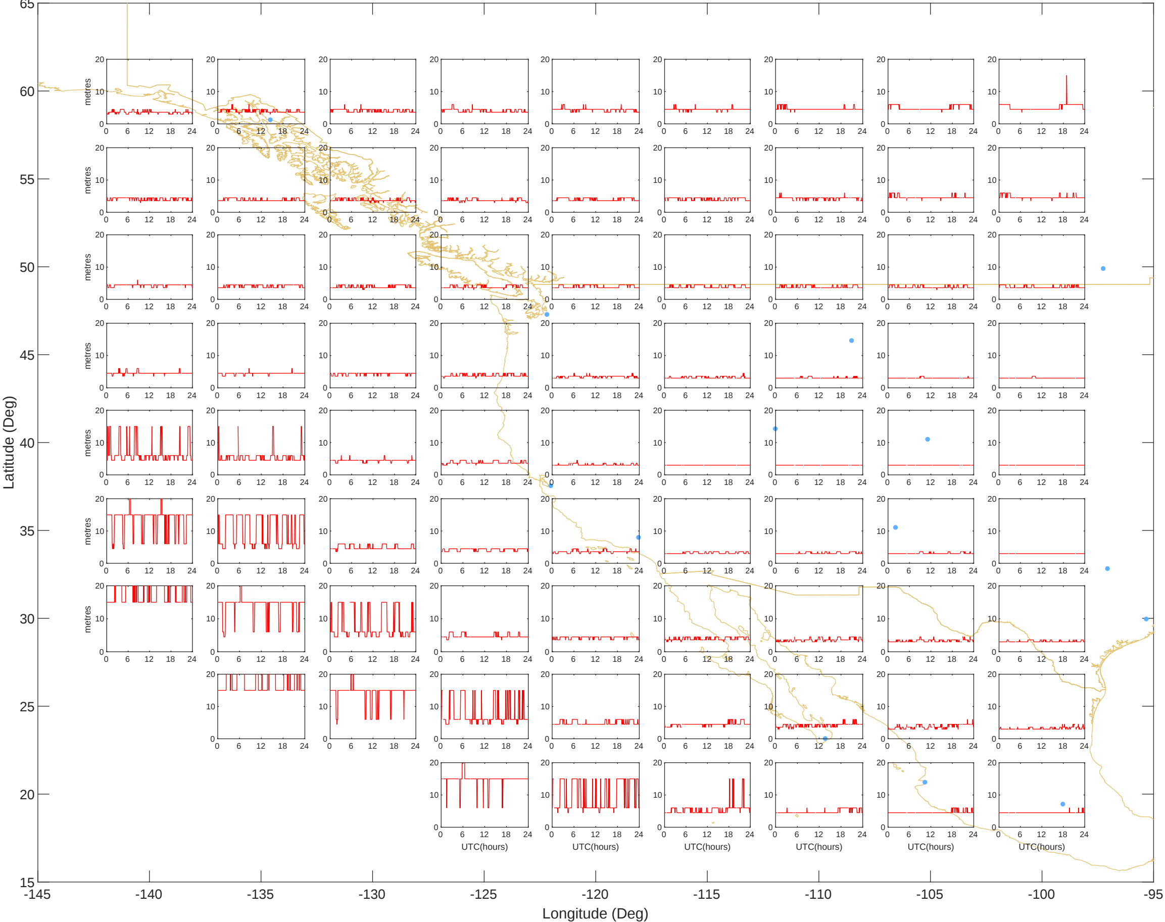
GIVEs - West (04-Oct-2025) @UNB-WAASLAB
