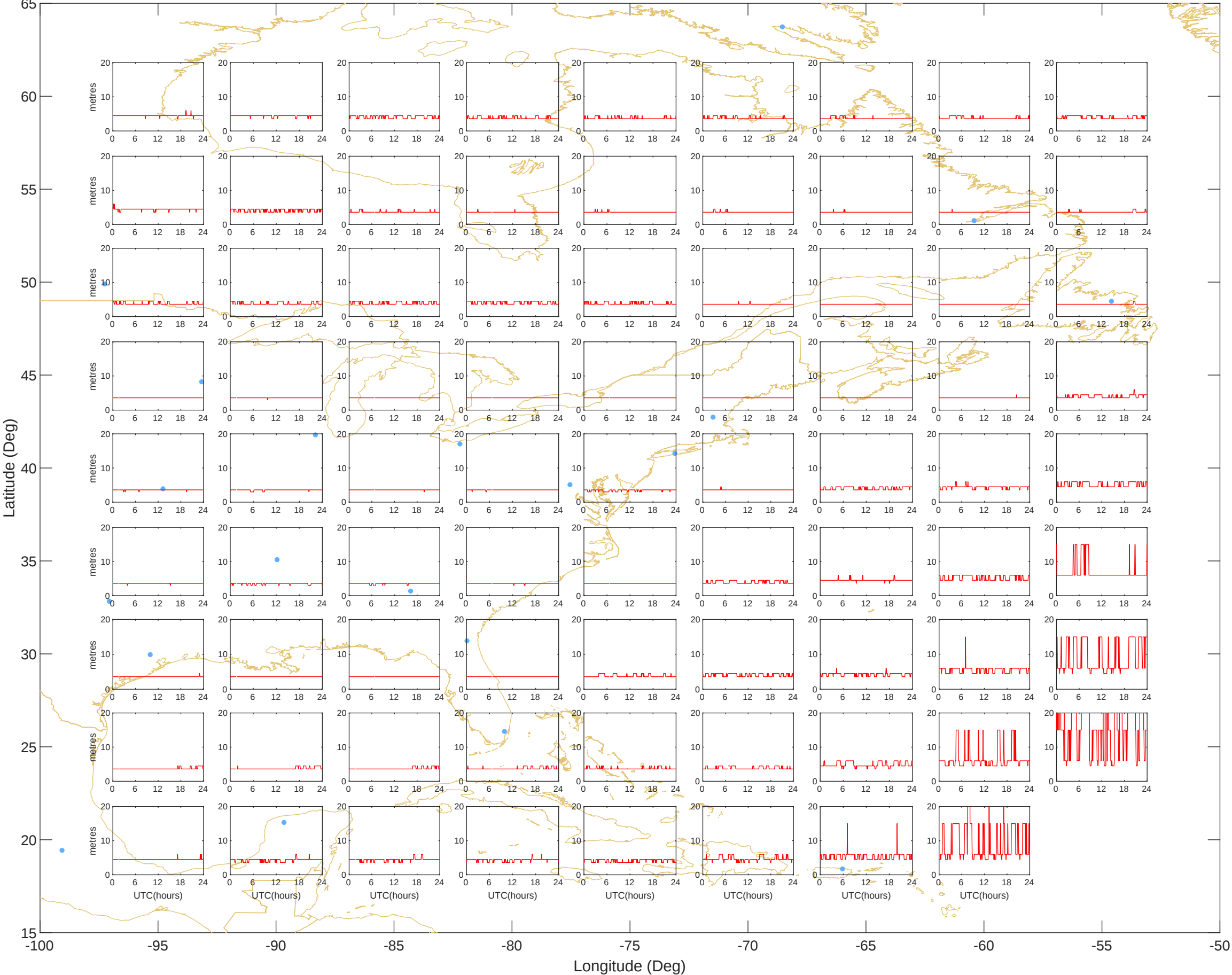
GIVEs - East (16-Aug-2026) @UNB-WAASLAB
