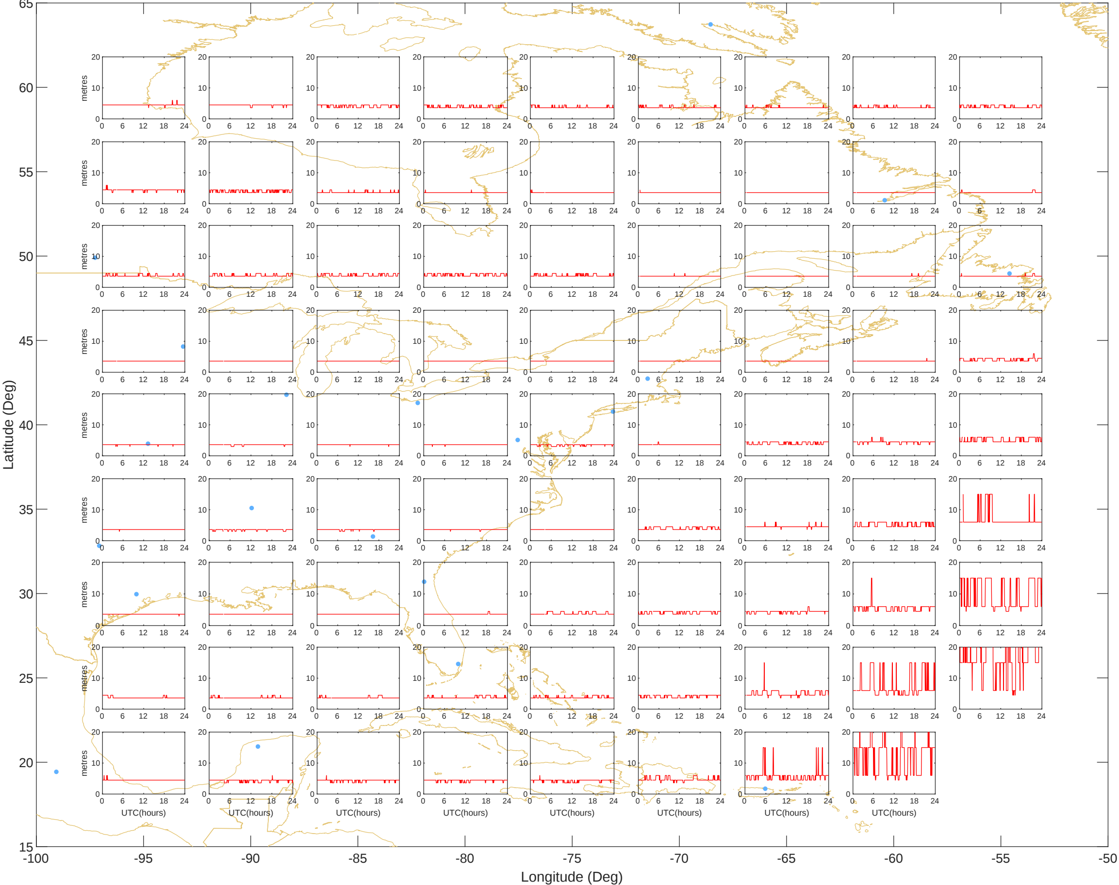
GIVEs - East (01-Aug-2026) @UNB-WAASLAB
