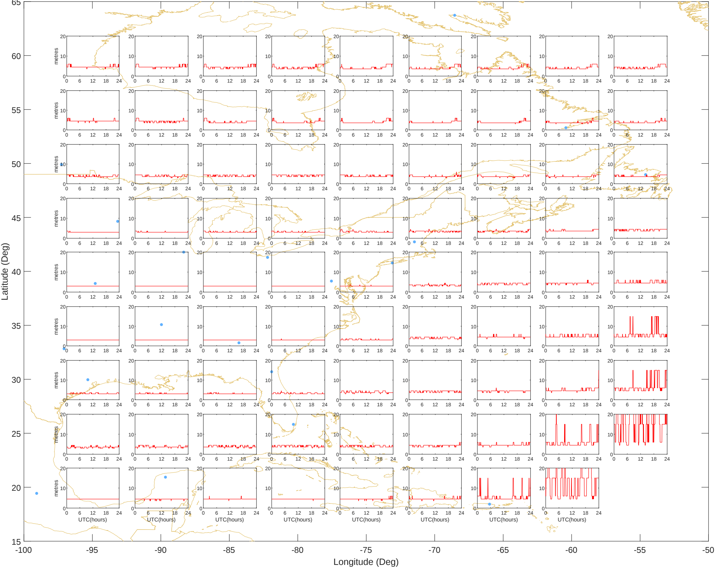
GIVEs - East (23-Feb-2026) @UNB-WAASLAB
