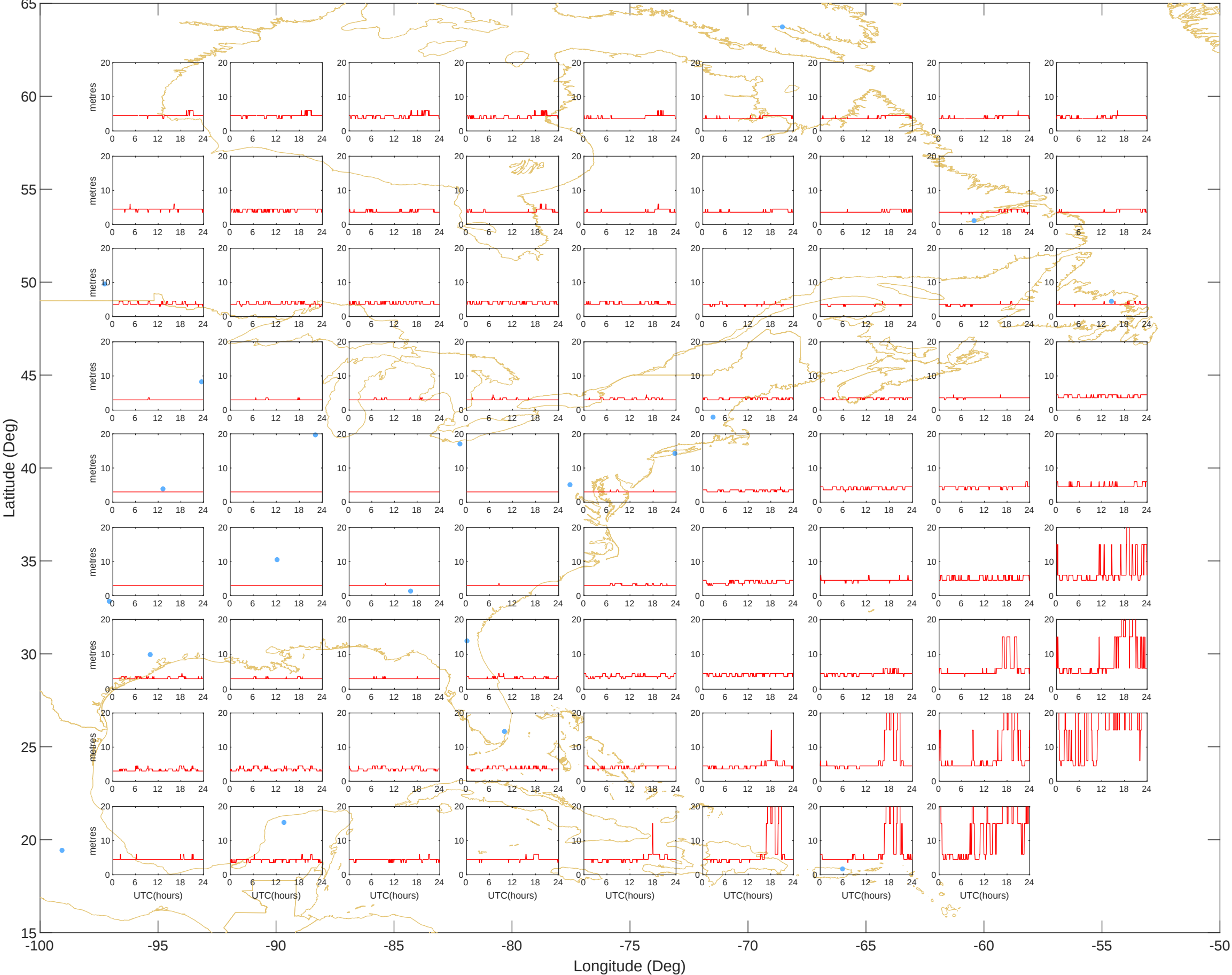
GIVEs - East (25-Dec-2025) @UNB-WAASLAB
