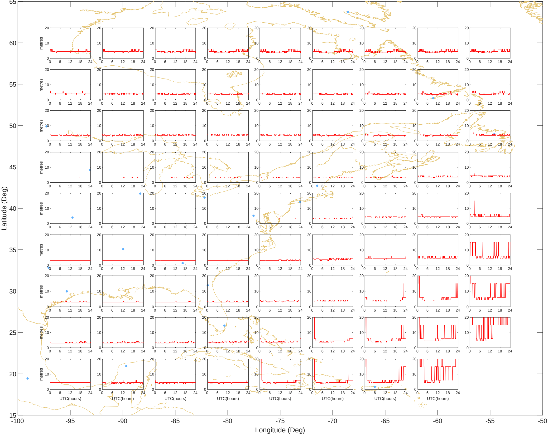
GIVEs - East (11-Nov-2025) @UNB-WAASLAB
