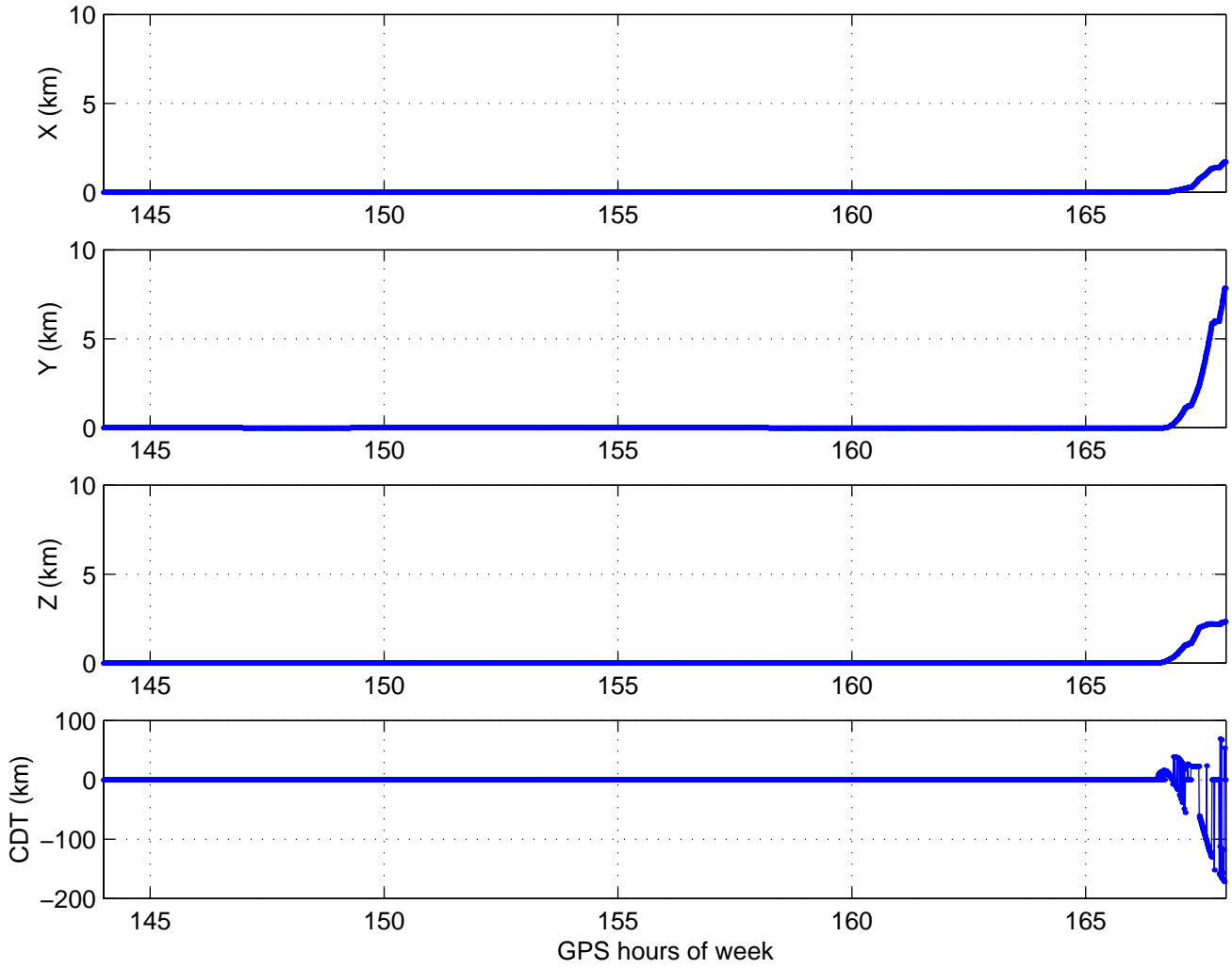
Pseudorange State Estimation – Divergence From Initial Solution: MDO1 (Texas) 01/07/28
