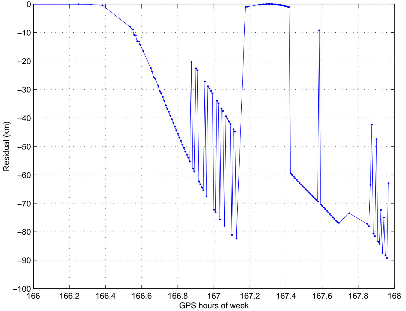
PRN 22 Pseudorange Residuals: MDO1 (Texas) 01/07/28
