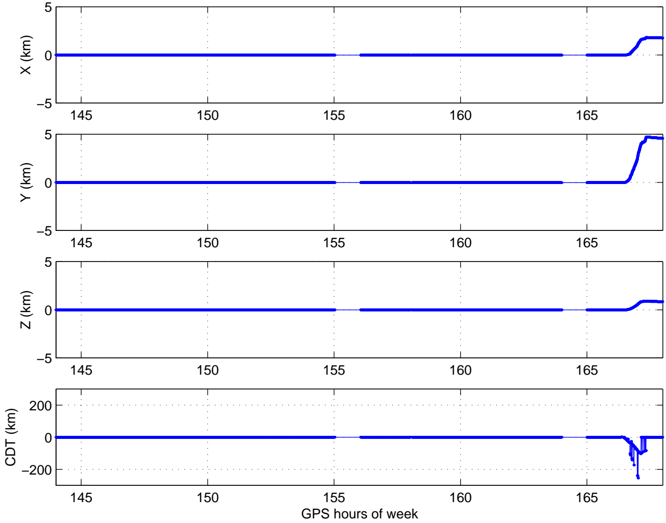
Pseudorange State Estimation – Divergence From Initial Solution: EISL (Easter Island) 01/07/28
