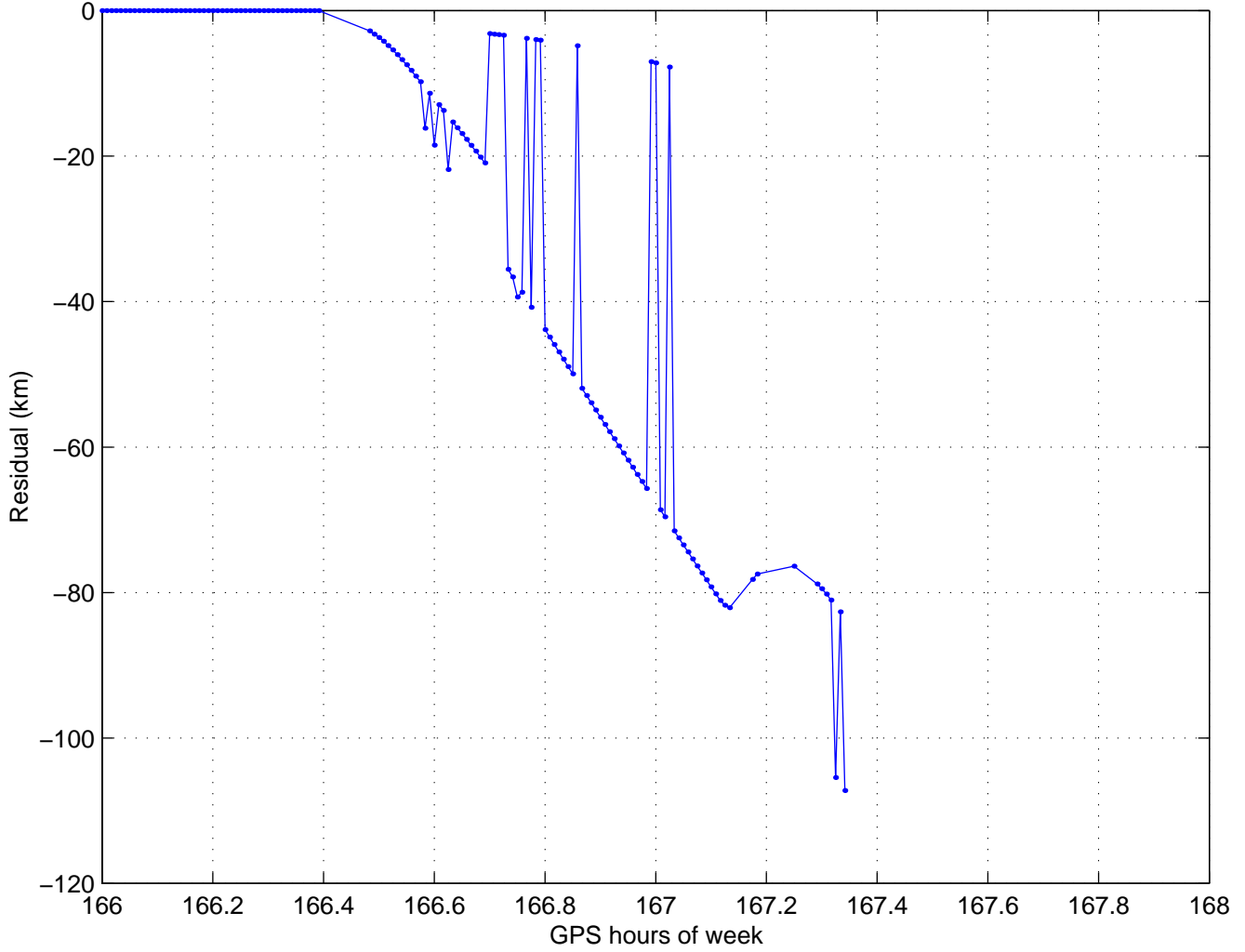
PRN 22 Pseudorange Residuals: EISL (Easter Island) 01/07/28
