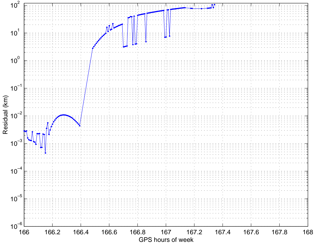
PRN 22 Pseudorange Residuals: EISL (Easter Island) 01/07/28
